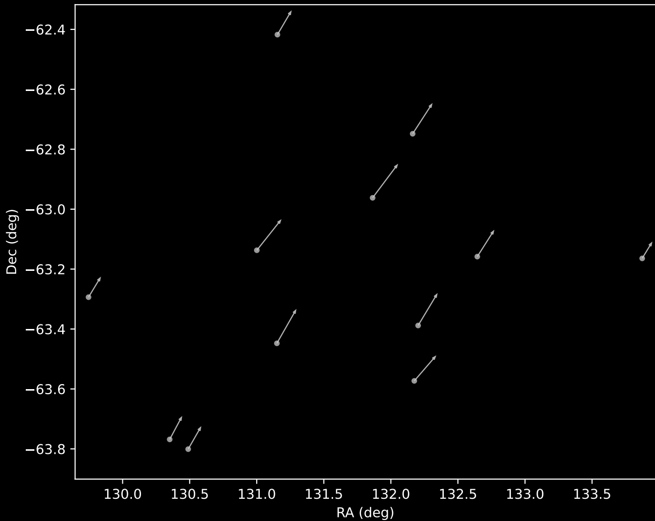
GALAH DR4 Cluster 15 Proper Motion Vectors (n=12)
