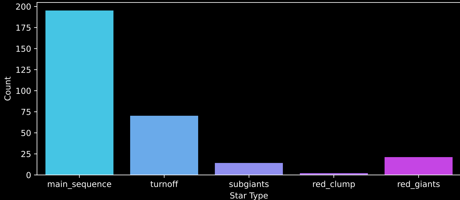
GALAH DR4 Field: [6960] Count plot of Star Type
