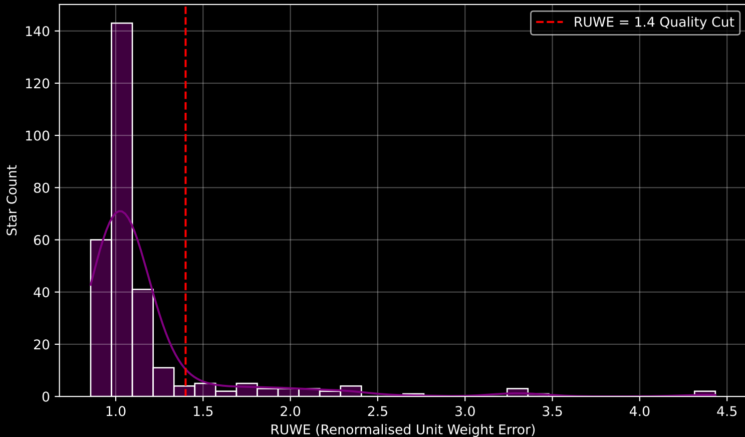
GALAH DR4 Field [6960] RUWE Distribution (n= 293)
