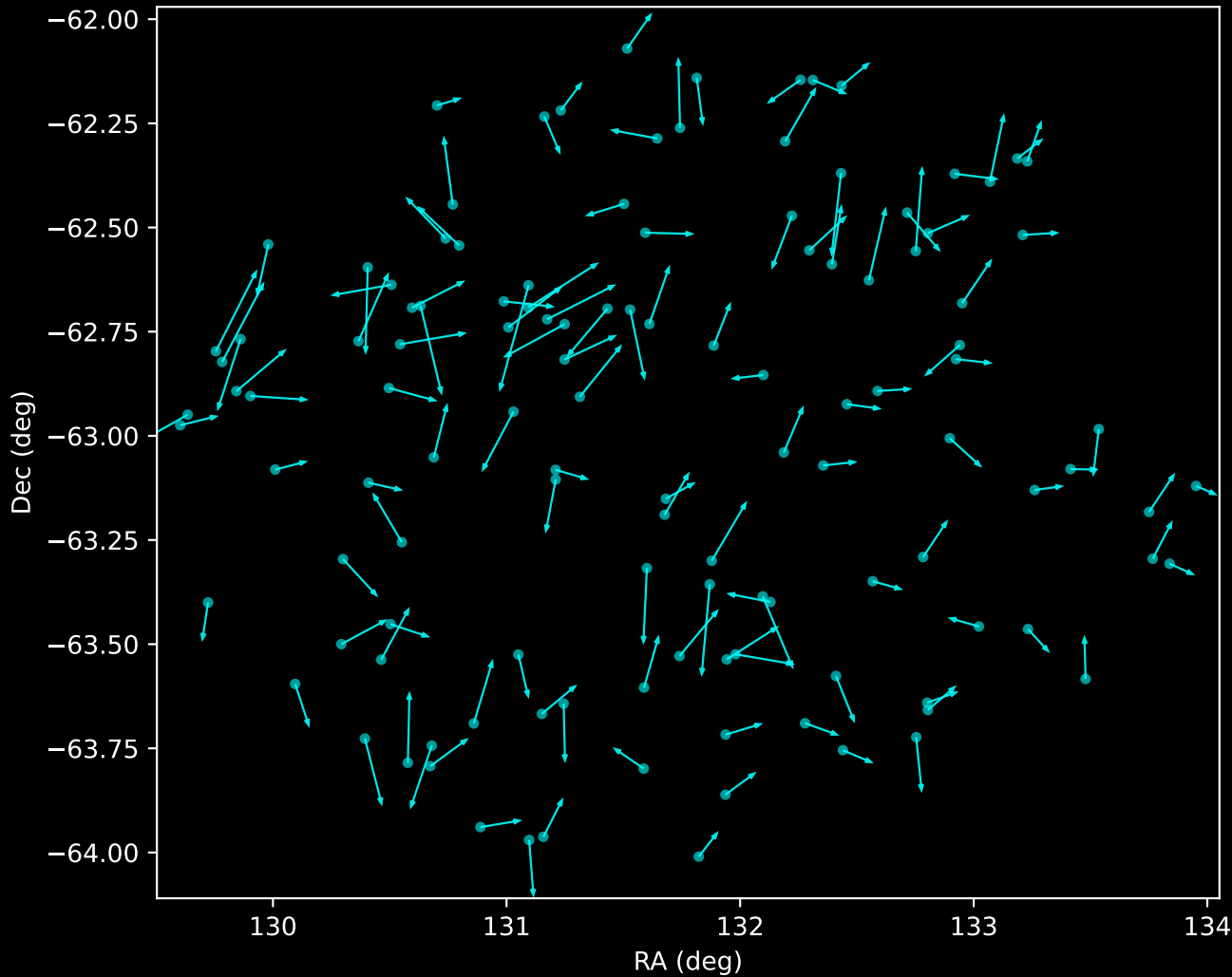
GALAH DR4 Noise Stream Proper Motion Vectors (n=122)
