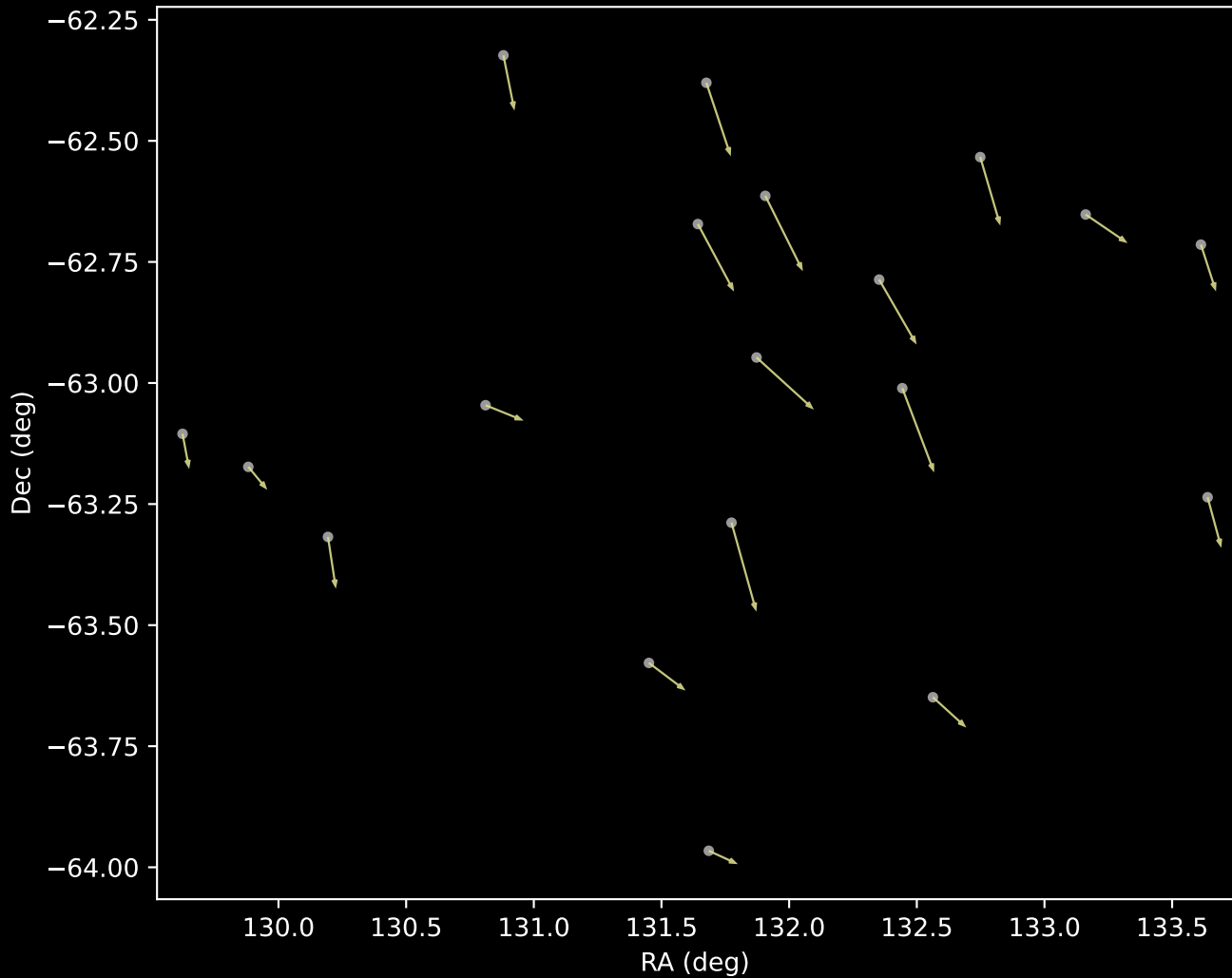
GALAH DR4 Cluster 17 Proper Motion Vectors (n=19)
