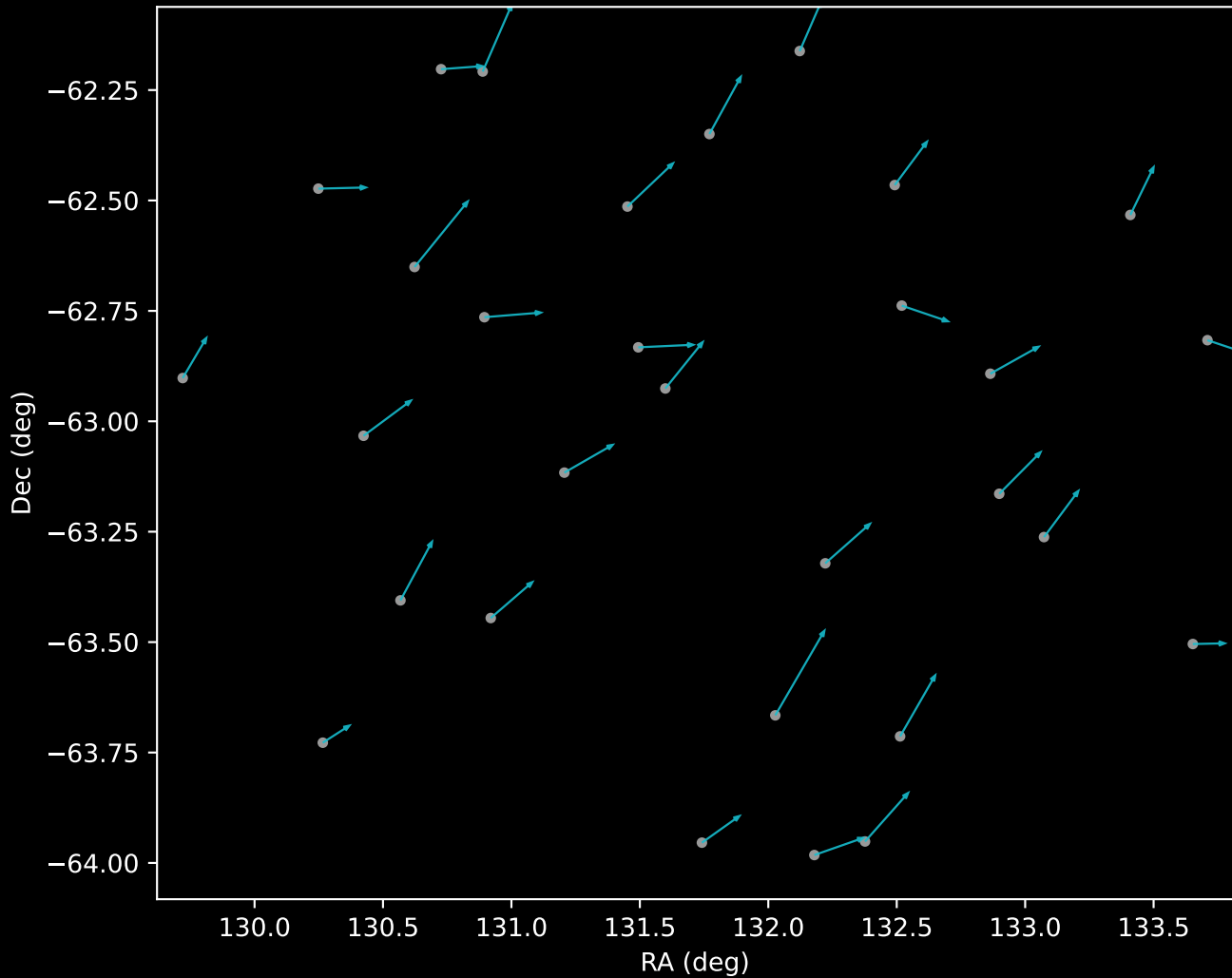
GALAH DR4 Cluster 18 Proper Motion Vectors (n=30)
