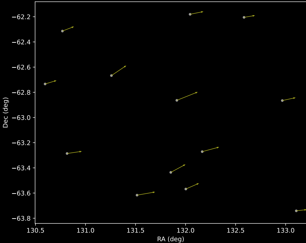
GALAH DR4 Cluster 16 Proper Motion Vectors (n=13)
